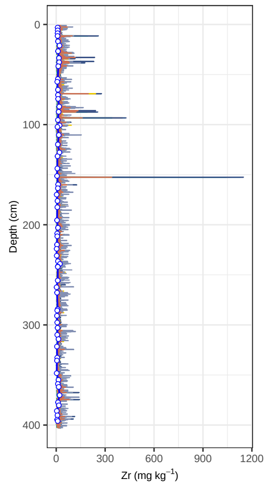
Site HER42PB – Zr (depth, all models)
