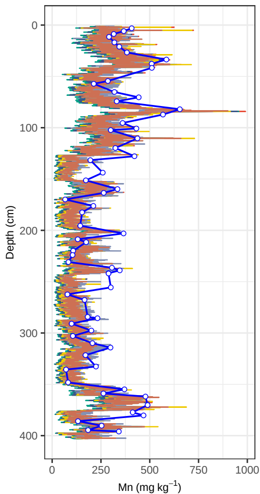
Site HER42PB – Mn (depth, all models)
