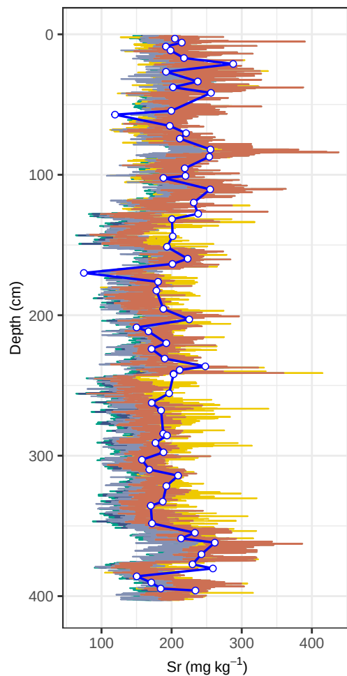
Site HER42PB – Sr (depth, all models)
