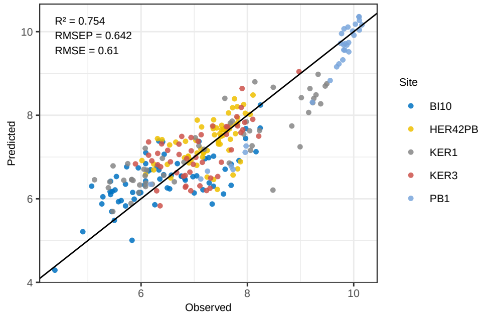
Ti PLS_LOO – Predicted vs Observed
