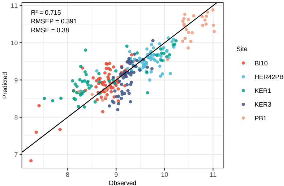
Ca PLS_kfold - Predicted vs Observed (log-space)
