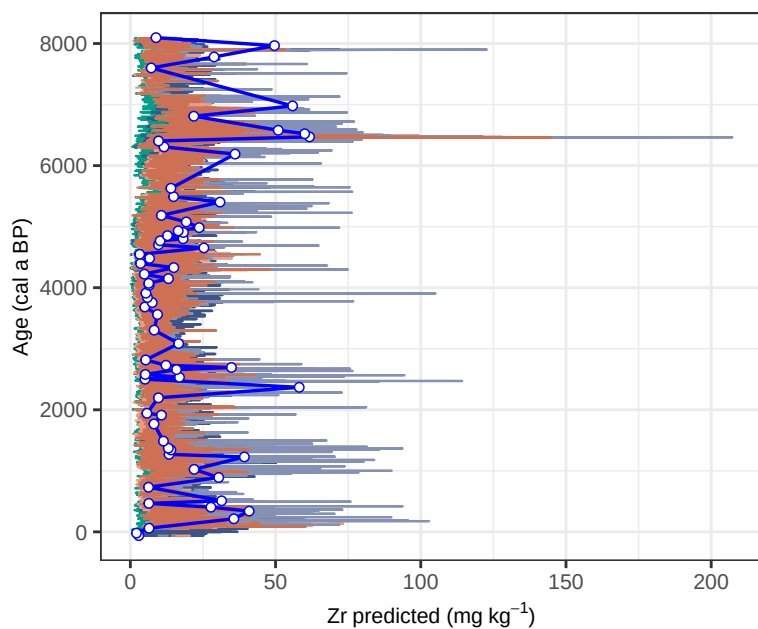
Site BI10 – Zr (age vs mg kg -1 , all)
