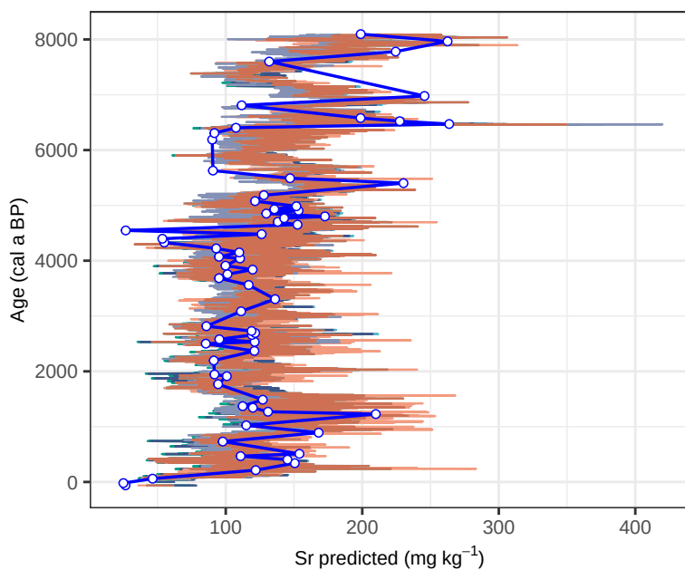
Site BI10 – Sr (age vs mg kg -1 , all)
