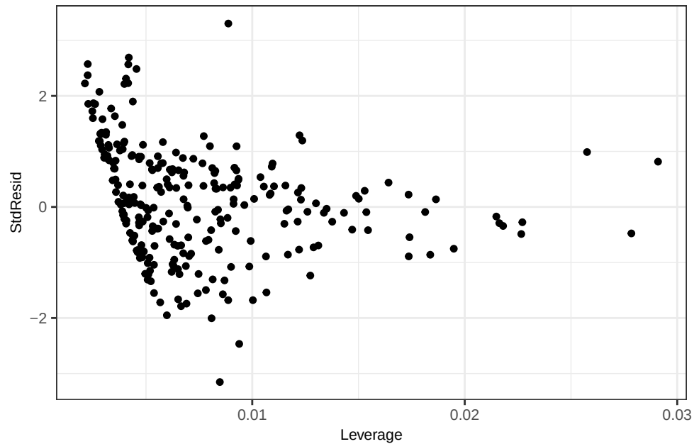
Mn OLS_weighted - Leverage Plot
