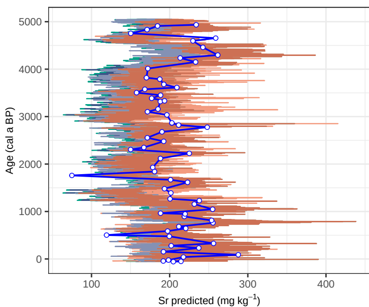
Site HER42PB – Sr (age vs mg kg -1 , all)
