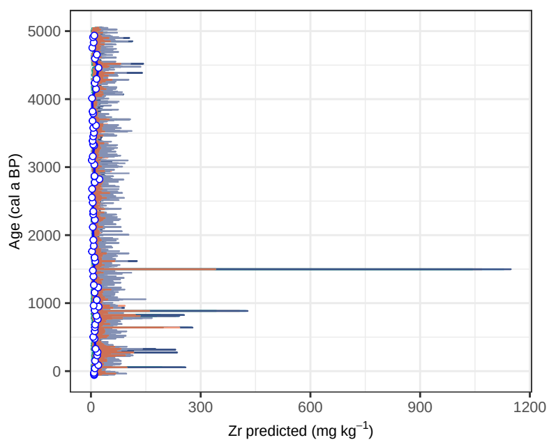
Site HER42PB – Zr (age vs mg kg -1 , all)
