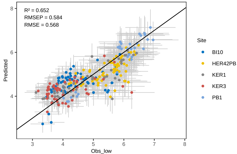
Mn PLS_kfold - Predicted vs Observed
