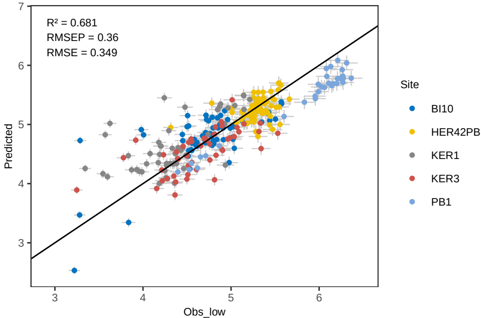
Sr PLS_LOO – Predicted vs Observed
