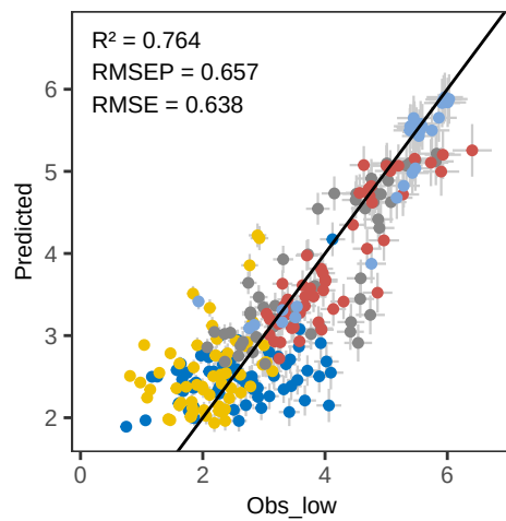
Zr PLS_LOO – Predicted vs Observed
