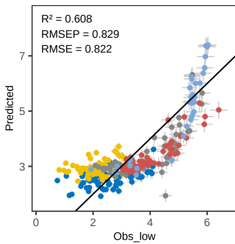
Zr WLS – Predicted vs Observed
