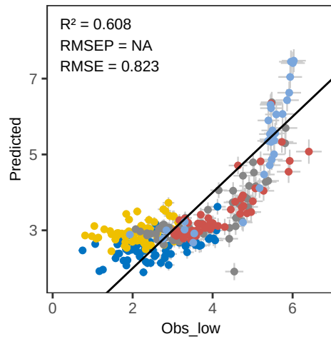
Zr RF – Predicted vs Observed
