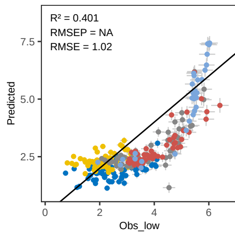
Zr WLS_weighted – Predicted vs Observed
