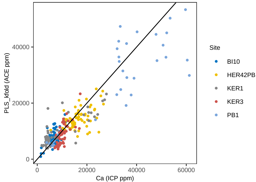
Ca PLS_kfold - ACE Pred vs Obs
