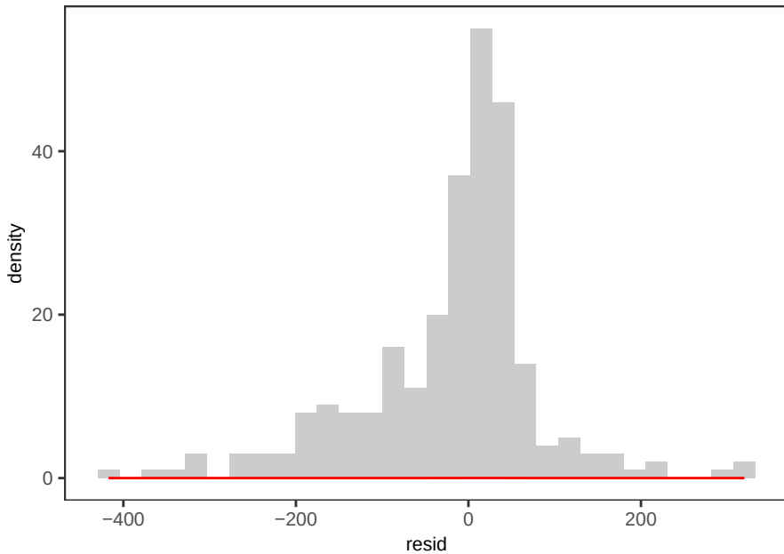
Mn Bayes - ACE Residuals
