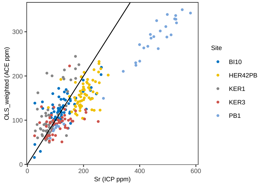
Sr OLS_weighted - ACE Pred vs Obs
