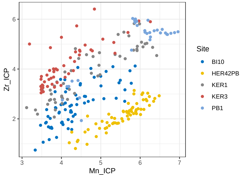
ICP relationship: Mn_ICP vs Zr_ICP
