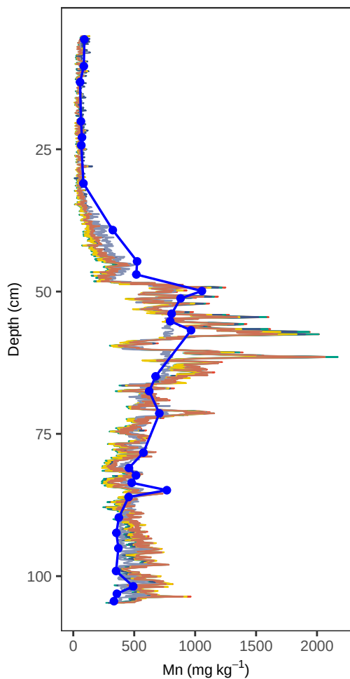
Site PB1 – Mn (depth, all models)
