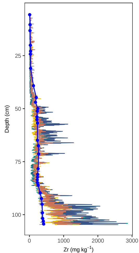
Site PB1 – Zr (depth, all models)
