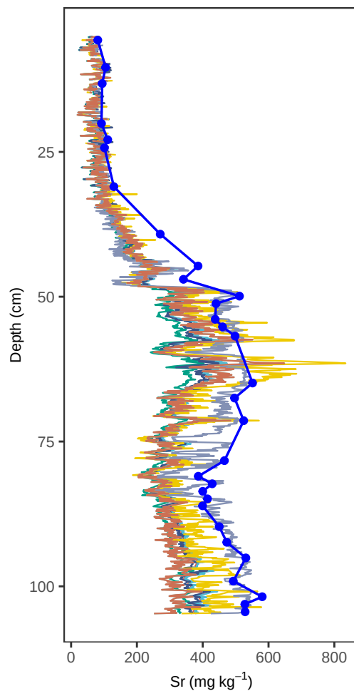
Site PB1 – Sr (depth, all models)
