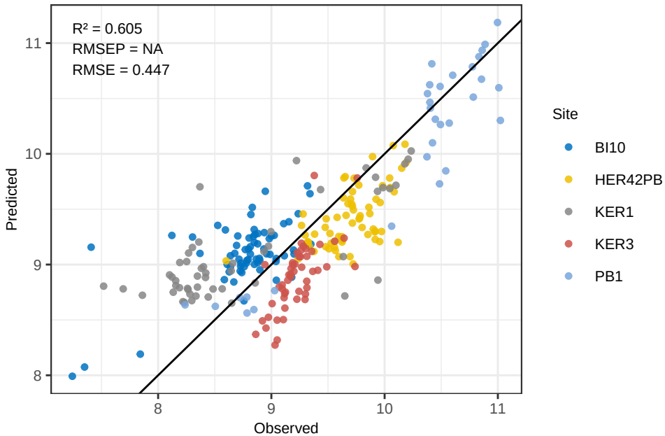
Ca WLS – Predicted vs Observed
