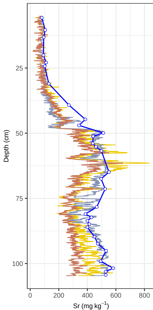
Site PB1 – Sr (depth, multivariate)
