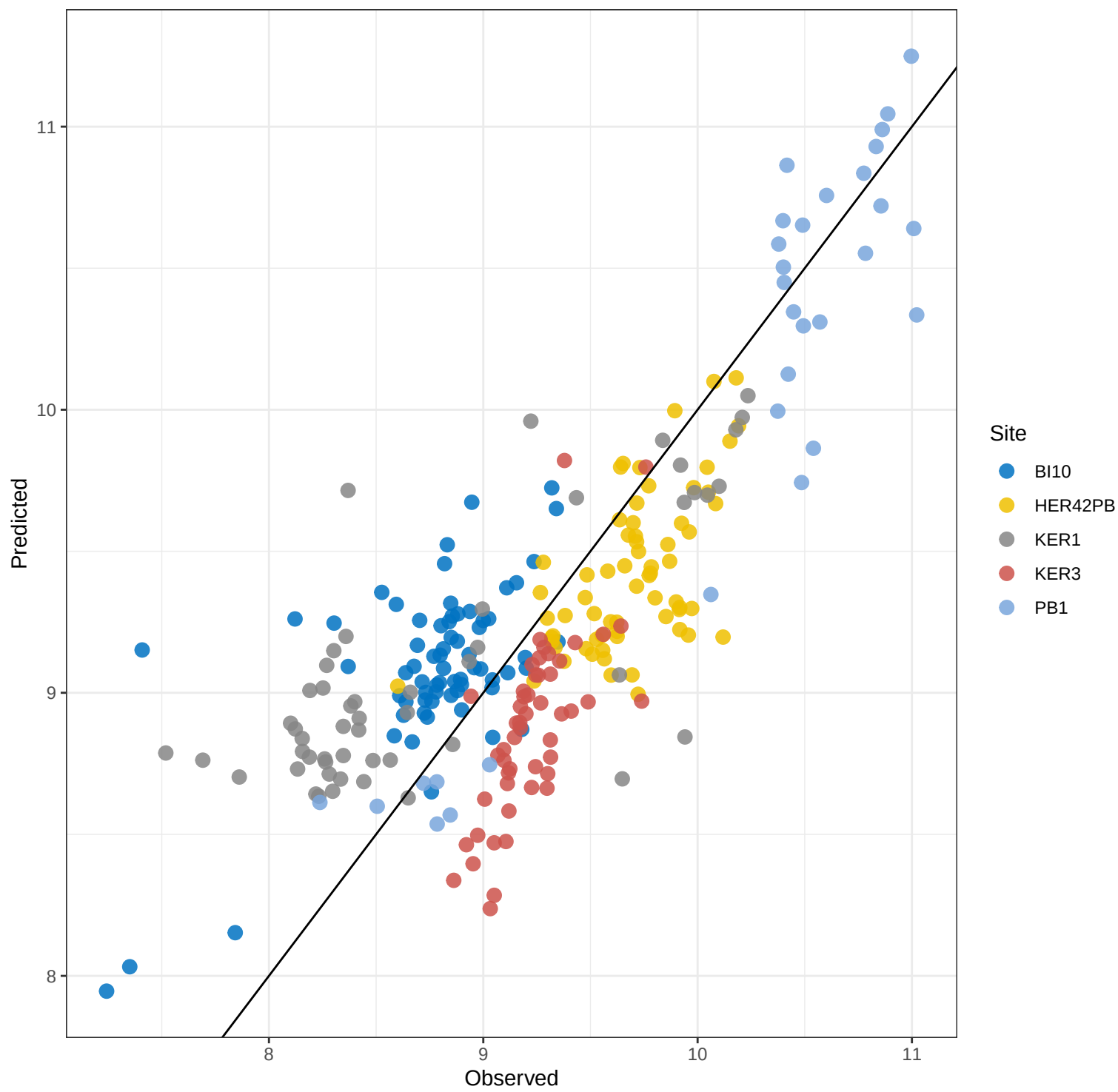
Ca PLS_LOO – Predicted vs Observed
