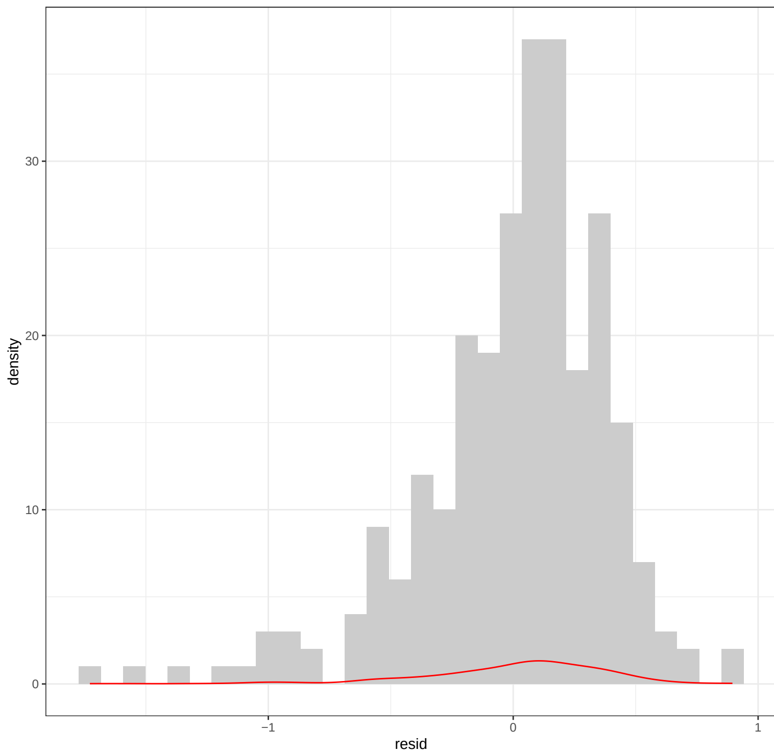
Sr Bayes - Residuals
