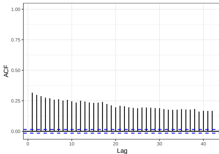
Series: ACE_xrf_qc$Cl
