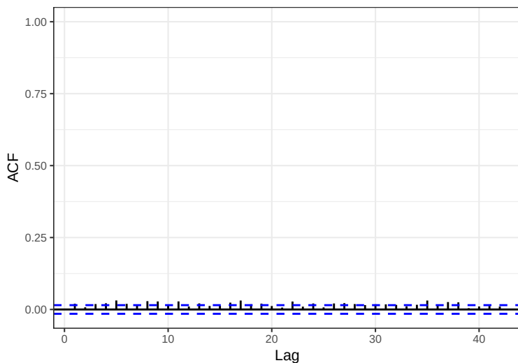
Series: ACE_xrf_qc$S
