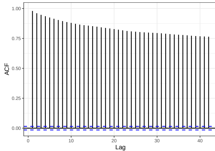
Series: ACE_xrf_qc$Fe
