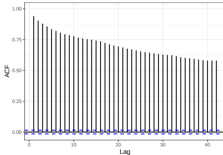
Series: ACE_xrf_qc$V
