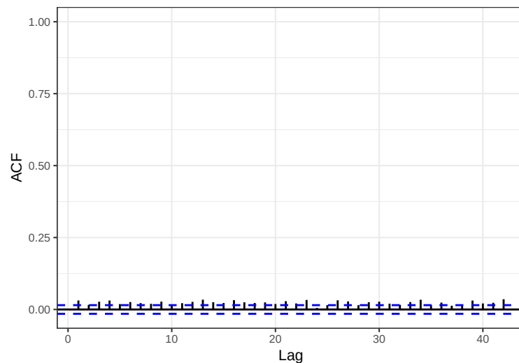
Series: ACE_xrf_qc$K
