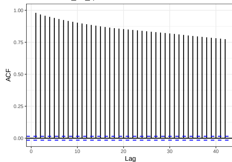
Series: ACE_xrf_qc$Zr
