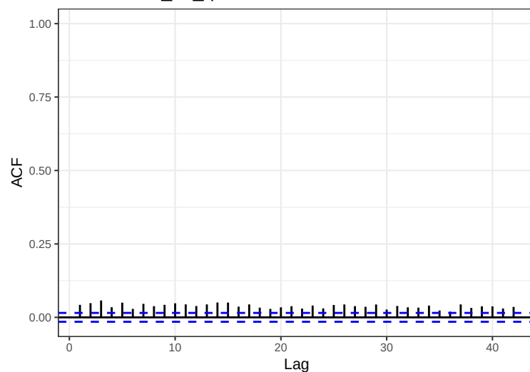
Series: ACE_xrf_qc$Sr
