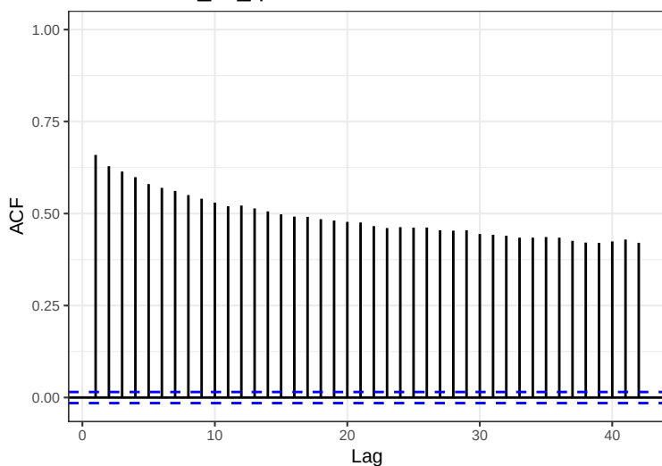
Series: ACE_xrf_qc$Zn
