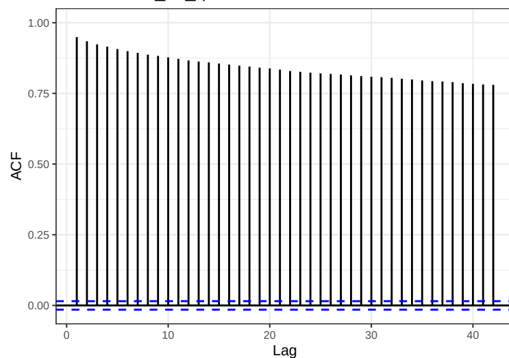
Series: ACE_xrf_qc$Mo_inc
