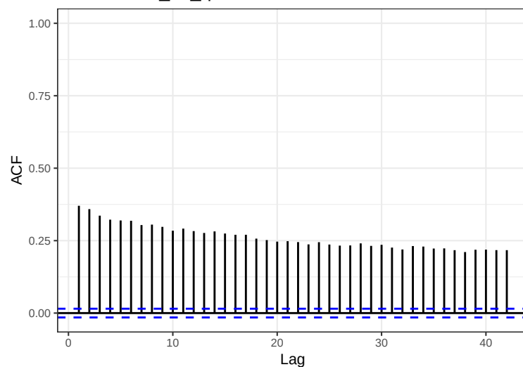
Series: ACE_xrf_qc$Se
