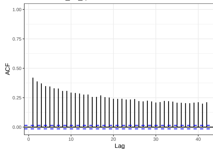
Series: ACE_xrf_qc$Br
