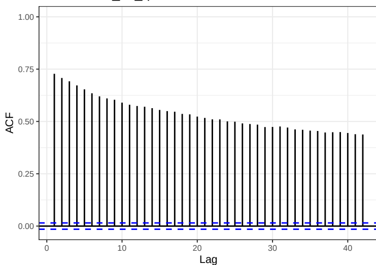
Series: ACE_xrf_qc$Ba
