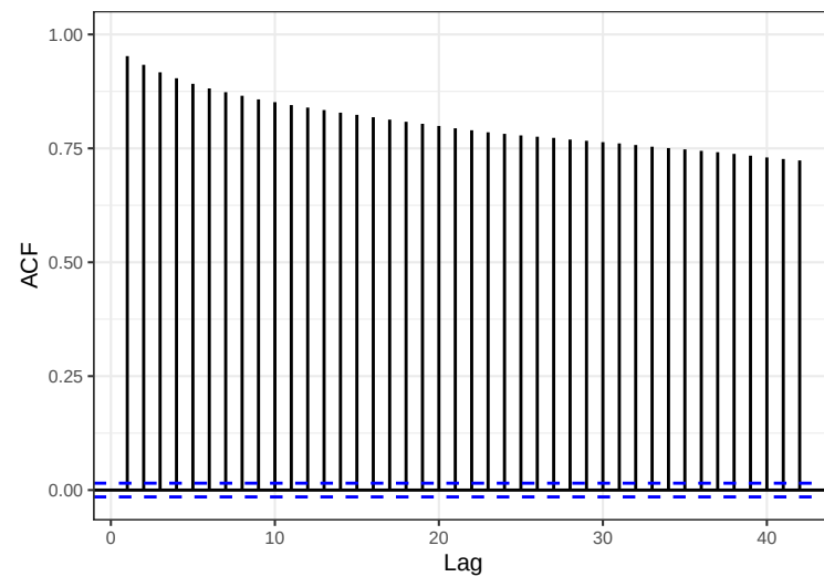
Series: ACE_xrf_qc$Mo_coh
