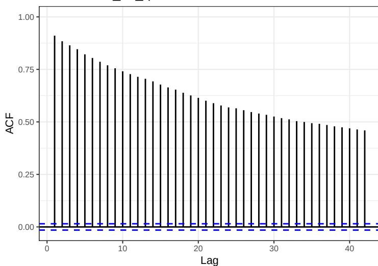
Series: ACE_xrf_qc$Rb
