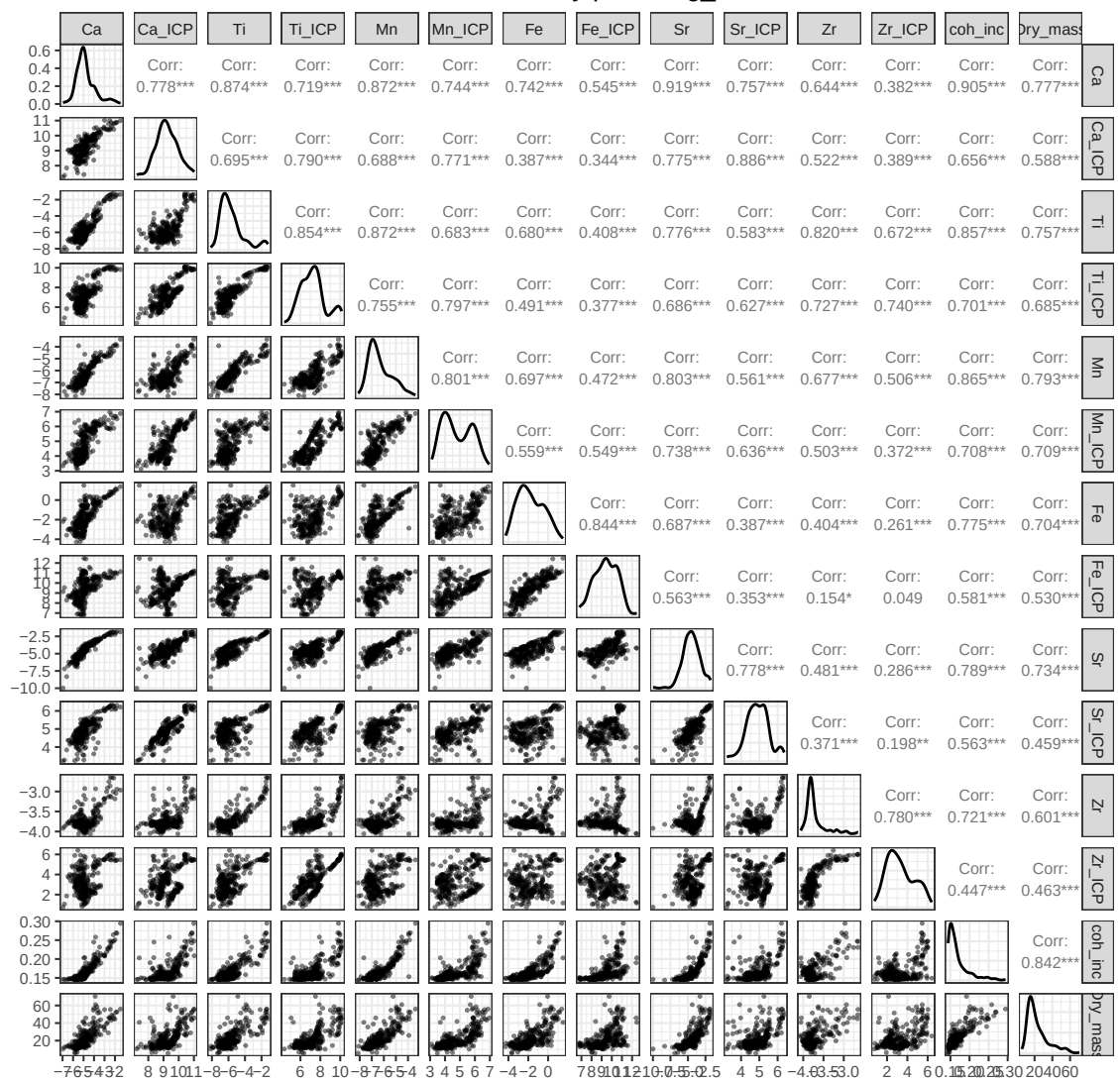
ACE XRF-CS &amp; ICPMS: Correlation-density plot – log_inc
