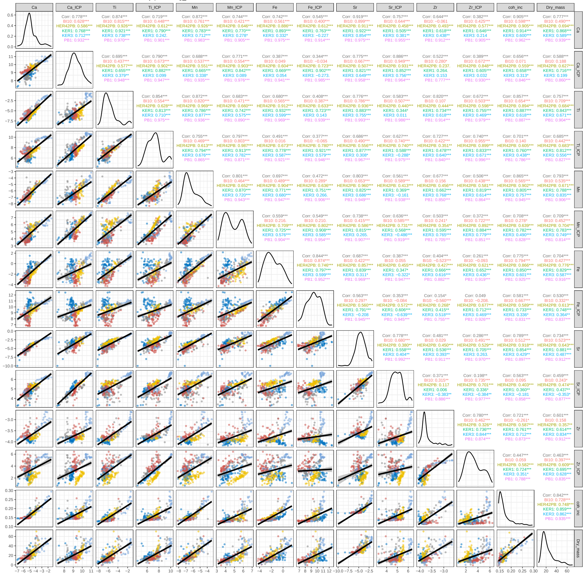
ACE XRF-CS & ICPMS: Correlation-density plot – log
