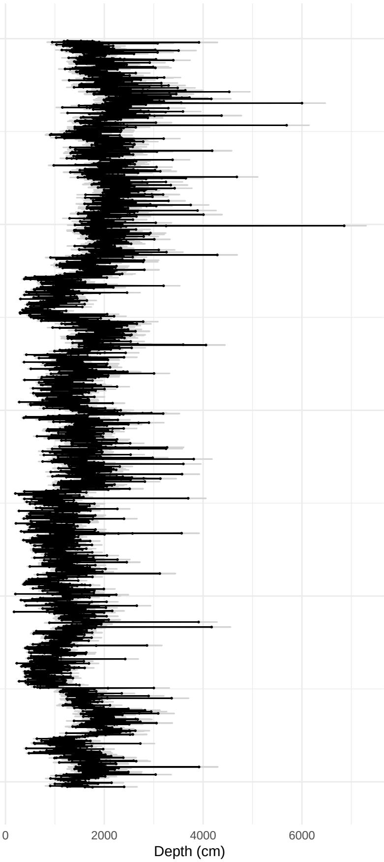
HER42PB: PLSR Ti Predictions with Confidence Int
