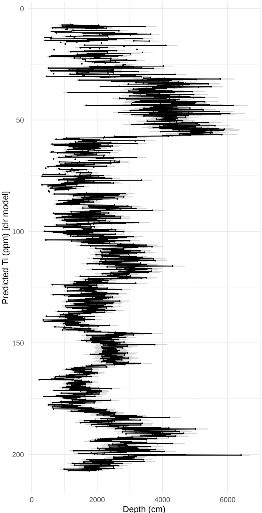
KER3: PLSR Ti Predictions with Confidence Interval
