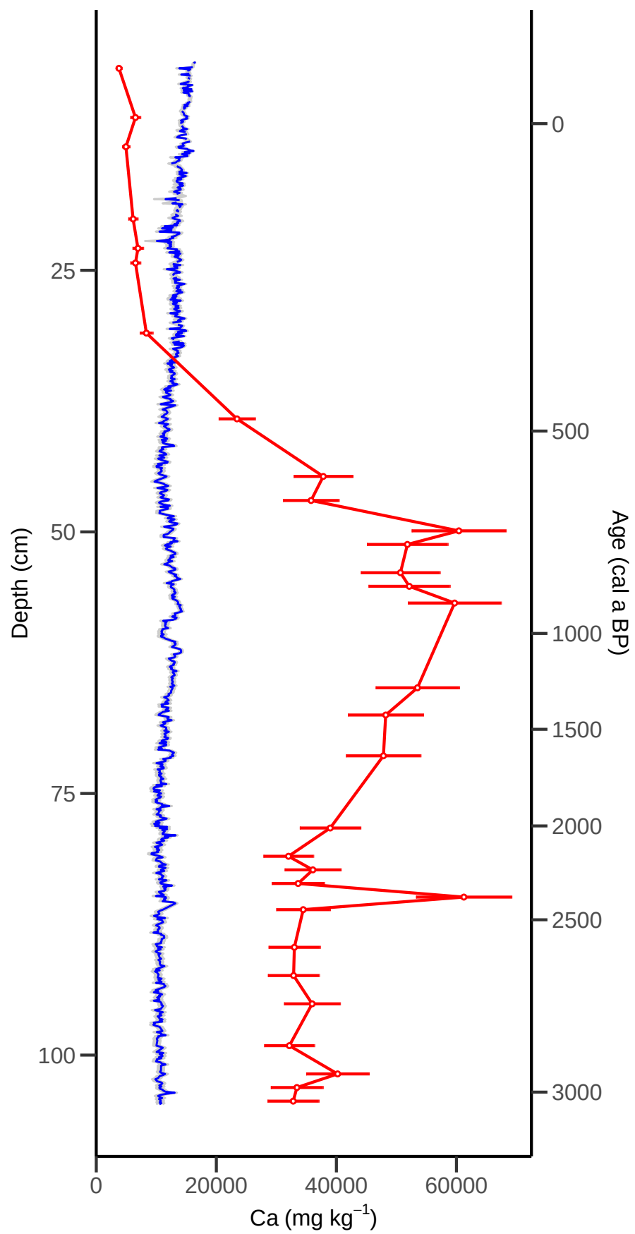
PB1: PLSR Ca Predictions with Confidence Intervals
