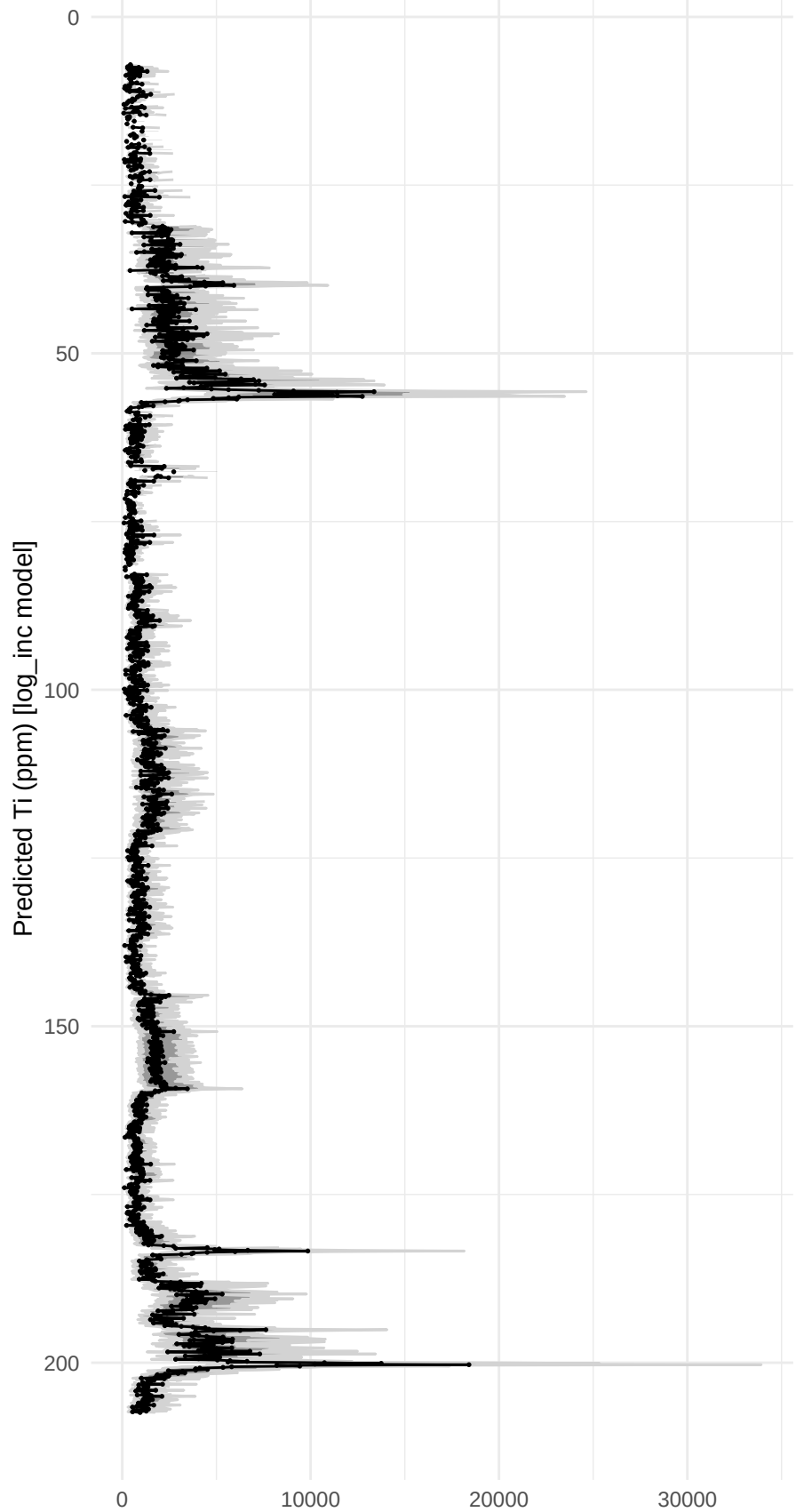
KER3: PLSR Ti Predictions with Confidence Interval
