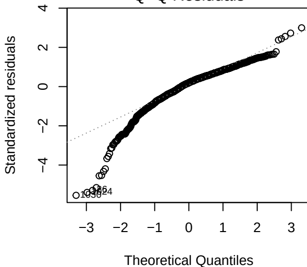
Q-Q Residuals
