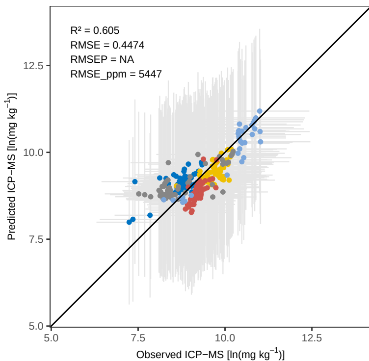
Ca WLS_weighted - Calibration
