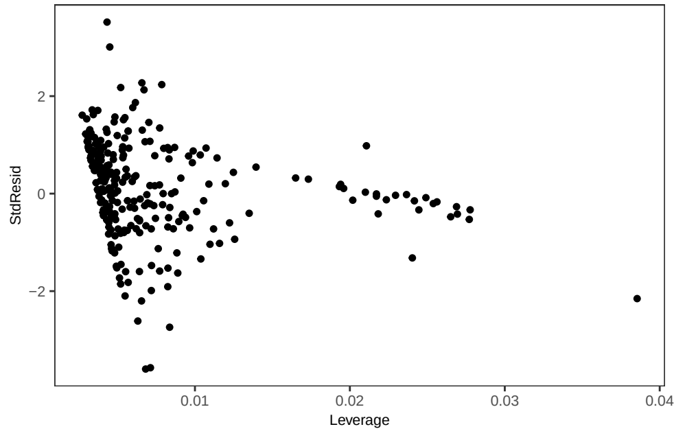
Ti OLS_weighted - Leverage
