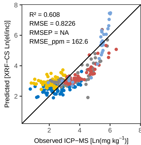
Zr RF – Pred vs Obs Training
