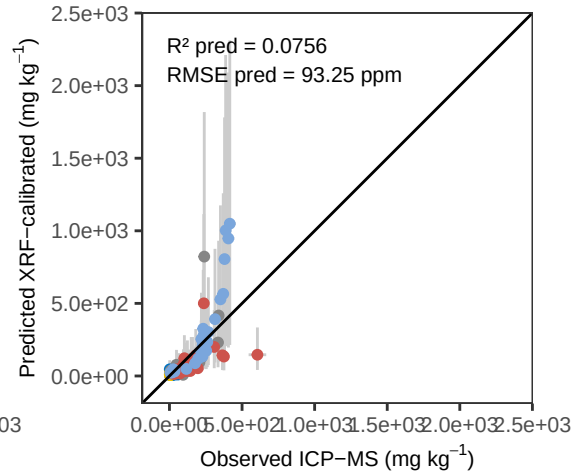
Zr PLS_kfold – External Validation
