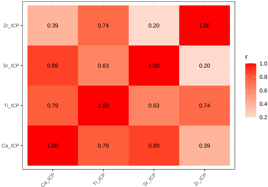
ICP log-space correlation matrix
