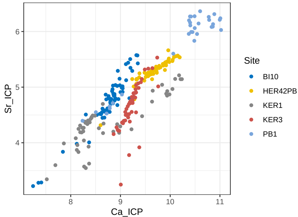
ICP relationship: Ca_ICP vs Sr_ICP
