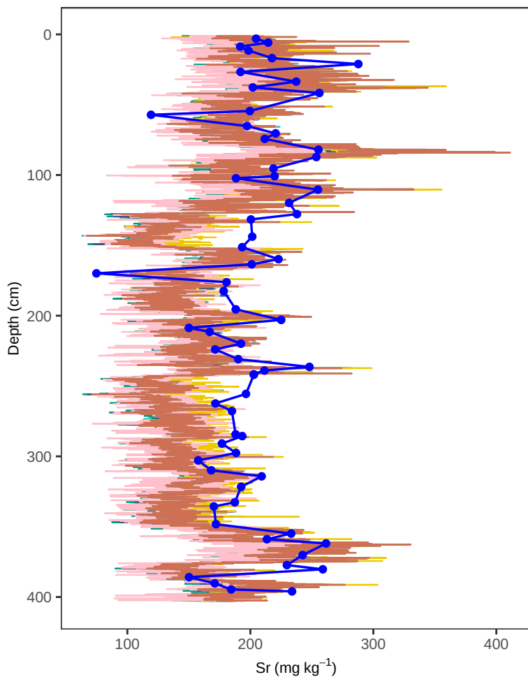
Site HER42PB – Sr (depth, all models)
