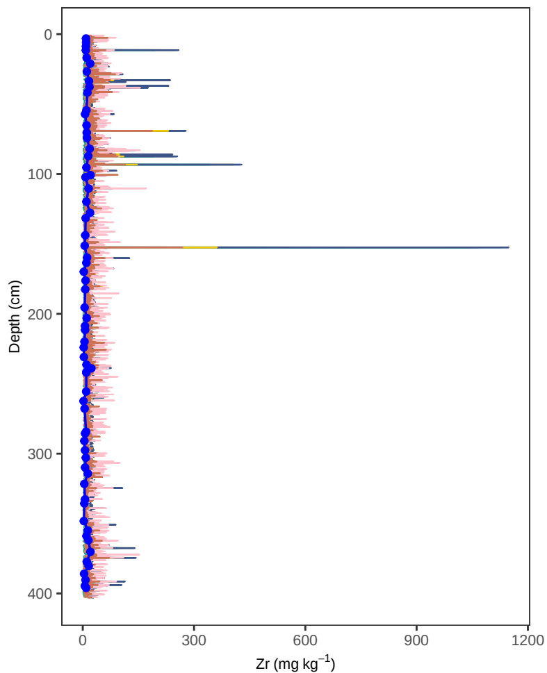
Site HER42PB – Zr (depth, all models)
