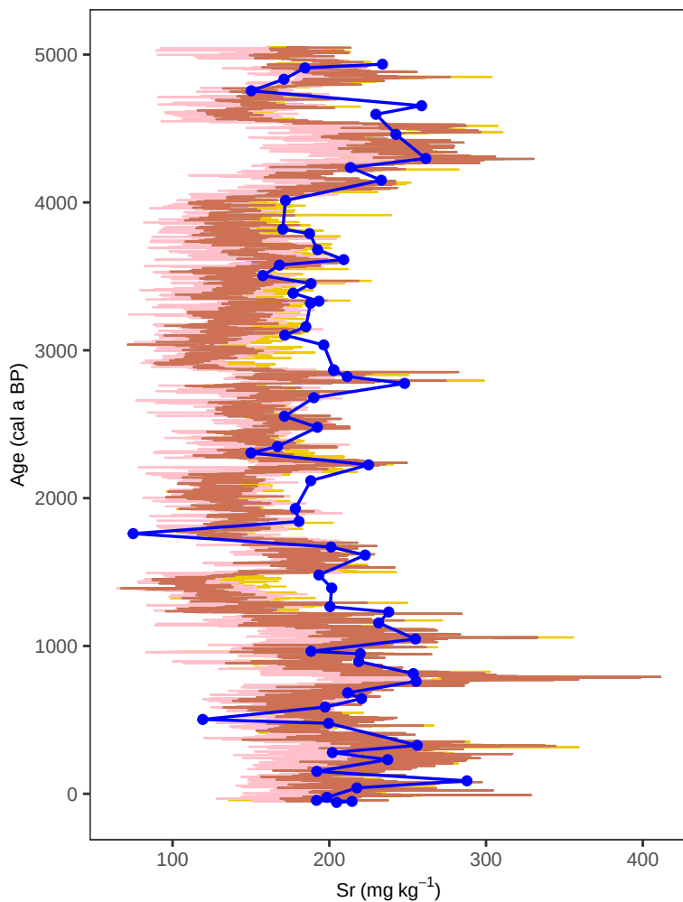
Site HER42PB – Sr (age, multivariate)
