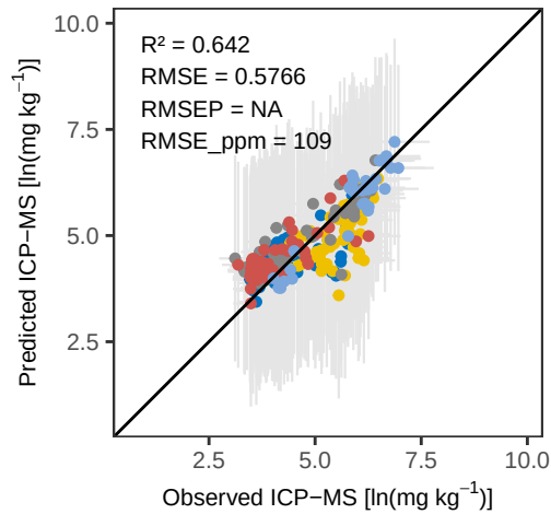
Mn Bayes – Calibration
