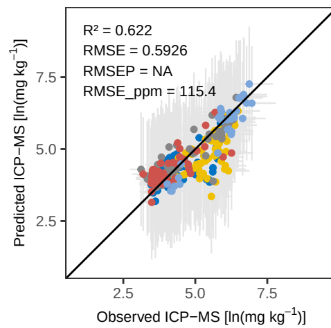
Mn WLS_weighted – Calibration
