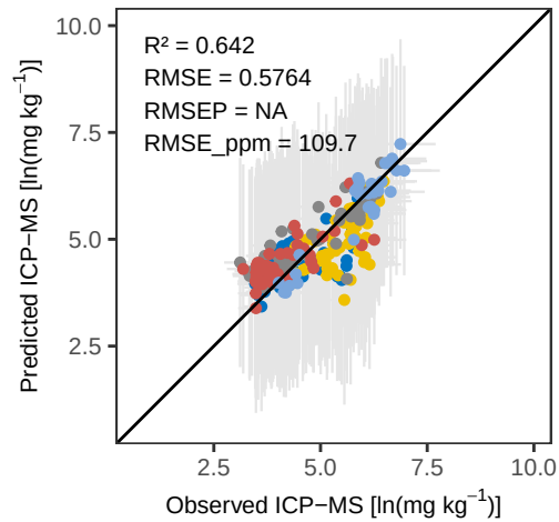
Mn RF – Calibration
