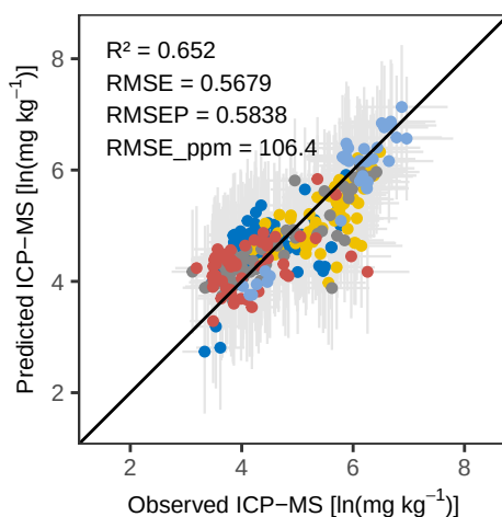
Mn PLS_kfold – Calibration
