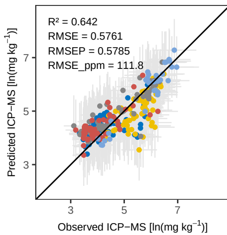
Mn WLS – Calibration
