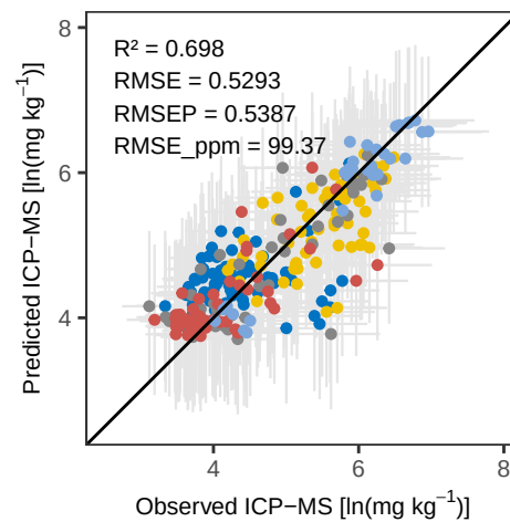
Mn PLS_LOO – Calibration
