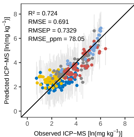
Zr PLS_kfold – Calibration
