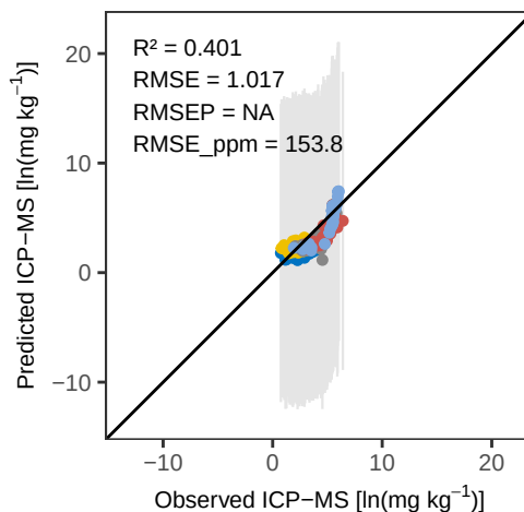
Zr WLS_weighted – Calibration
