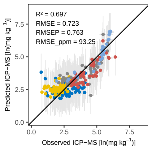
Zr PLS_kfold – Calibration
