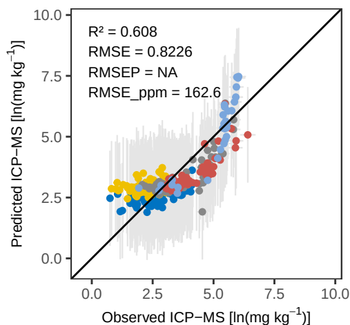
Zr RF – Calibration
