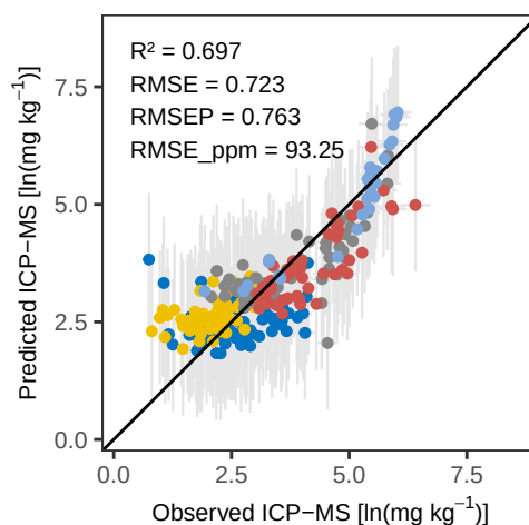
Zr PLS_LOO – Calibration
