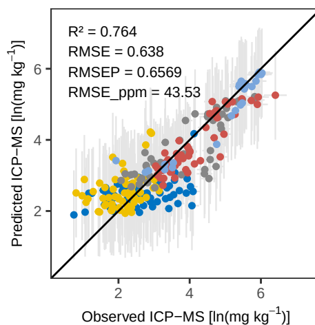
Zr PLS_LOO – Calibration
