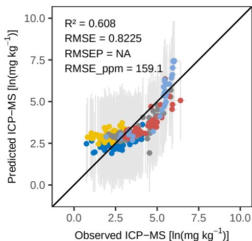
Zr Bayes – Calibration
