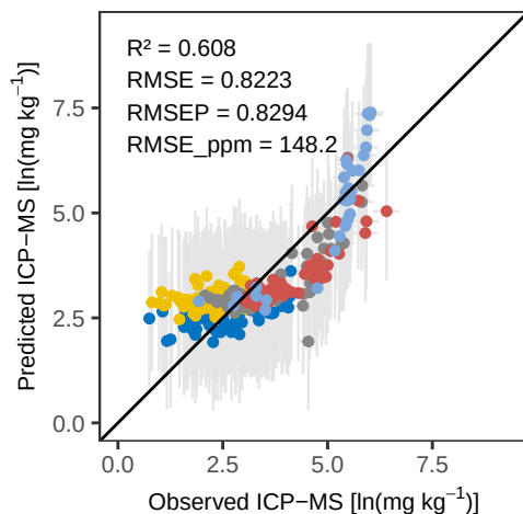
Zr WLS – Calibration
