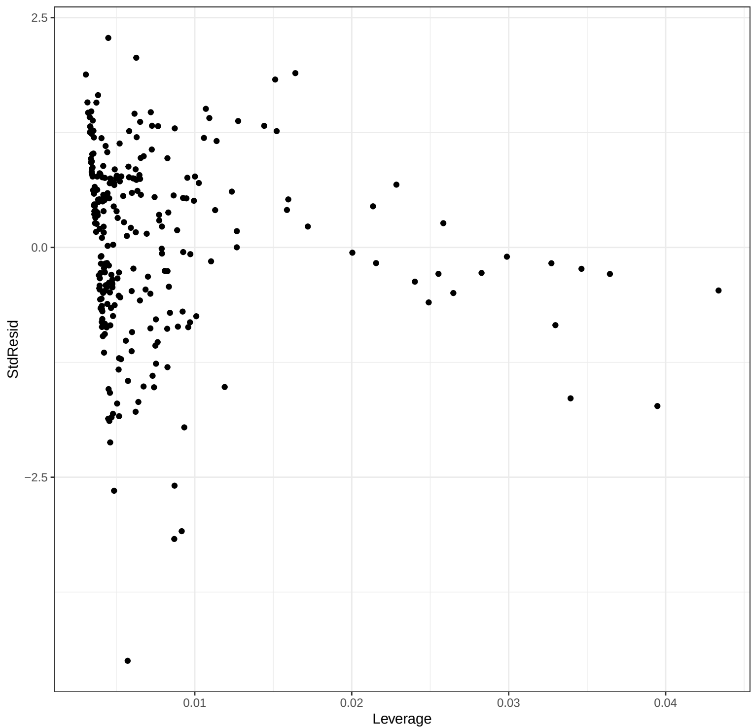
Ca OLS_weighted – Leverage Plot
