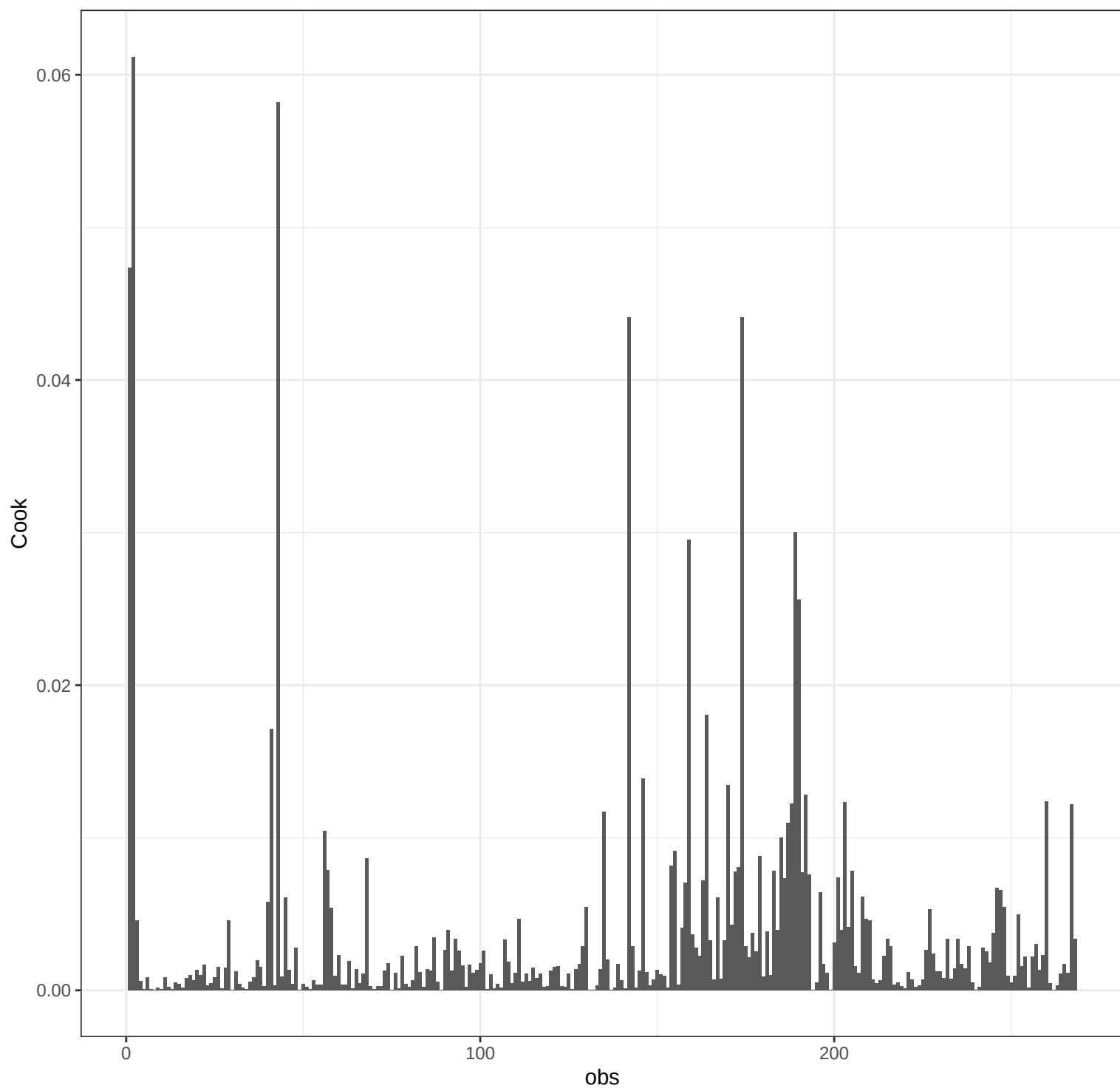
Ca OLS_weighted – Cook's Distance
