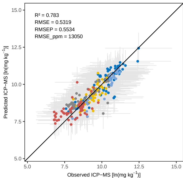
Fe Bayes – Calibration
