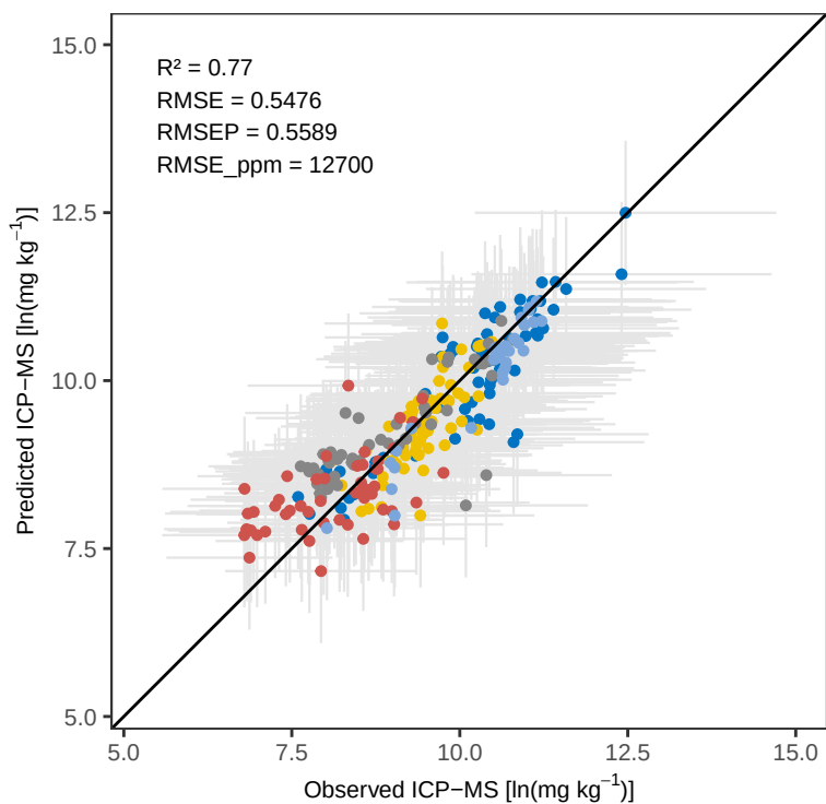
Fe PLS_kfold – Calibration
