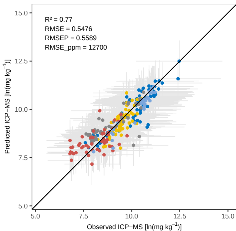
Fe PLS_LOO – Calibration
