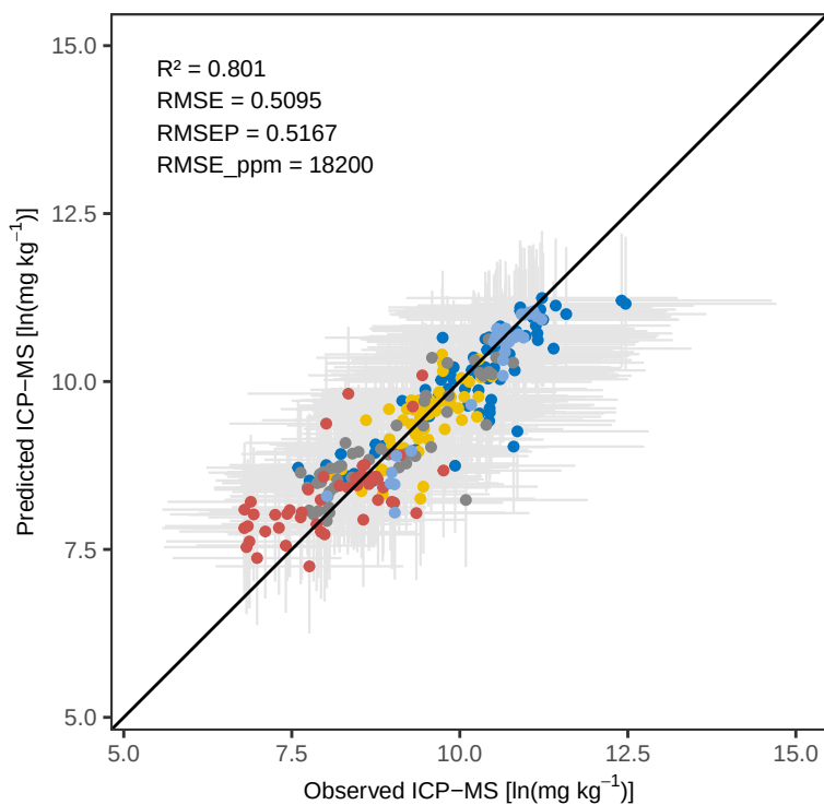
Fe RF – Calibration
