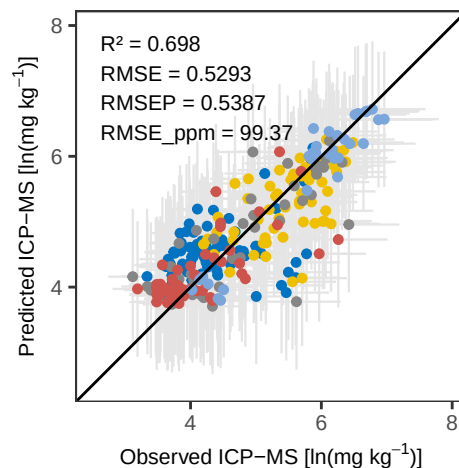
Mn PLS_LOO – Calibration
