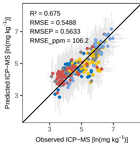
Mn PLS_kfold – Calibration
