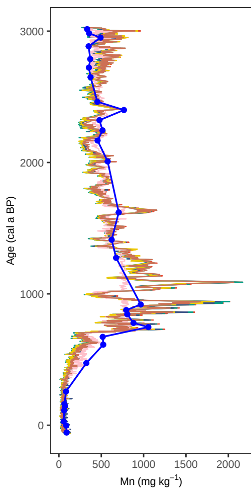
Site PB1 – Mn (age, all models)
