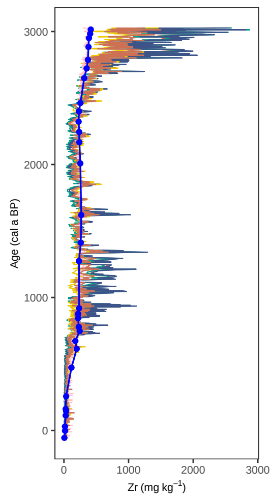
Site PB1 – Zr (age, all models)
