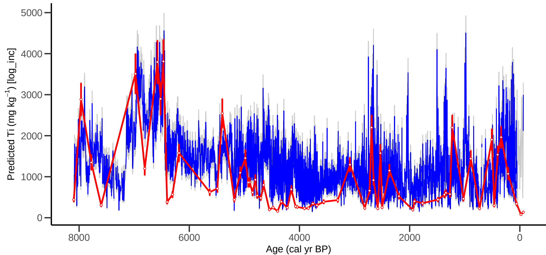
BI10: PLSR Ti Predictions with Confidence Interval (log_inc model)
