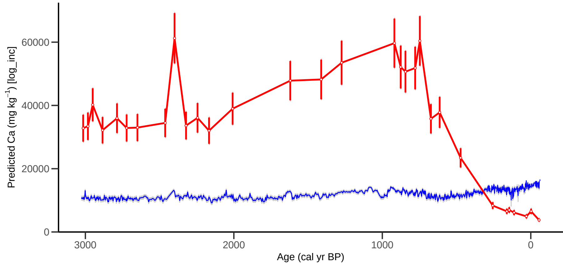
PB1: PLSR Ca Predictions with Confidence Interval (log_inc model)
