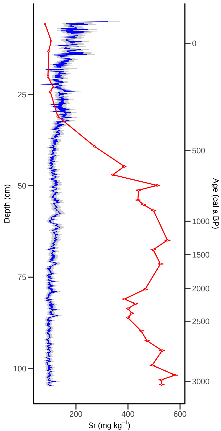
PB1: PLSR Sr Predictions with Confidence Interval
