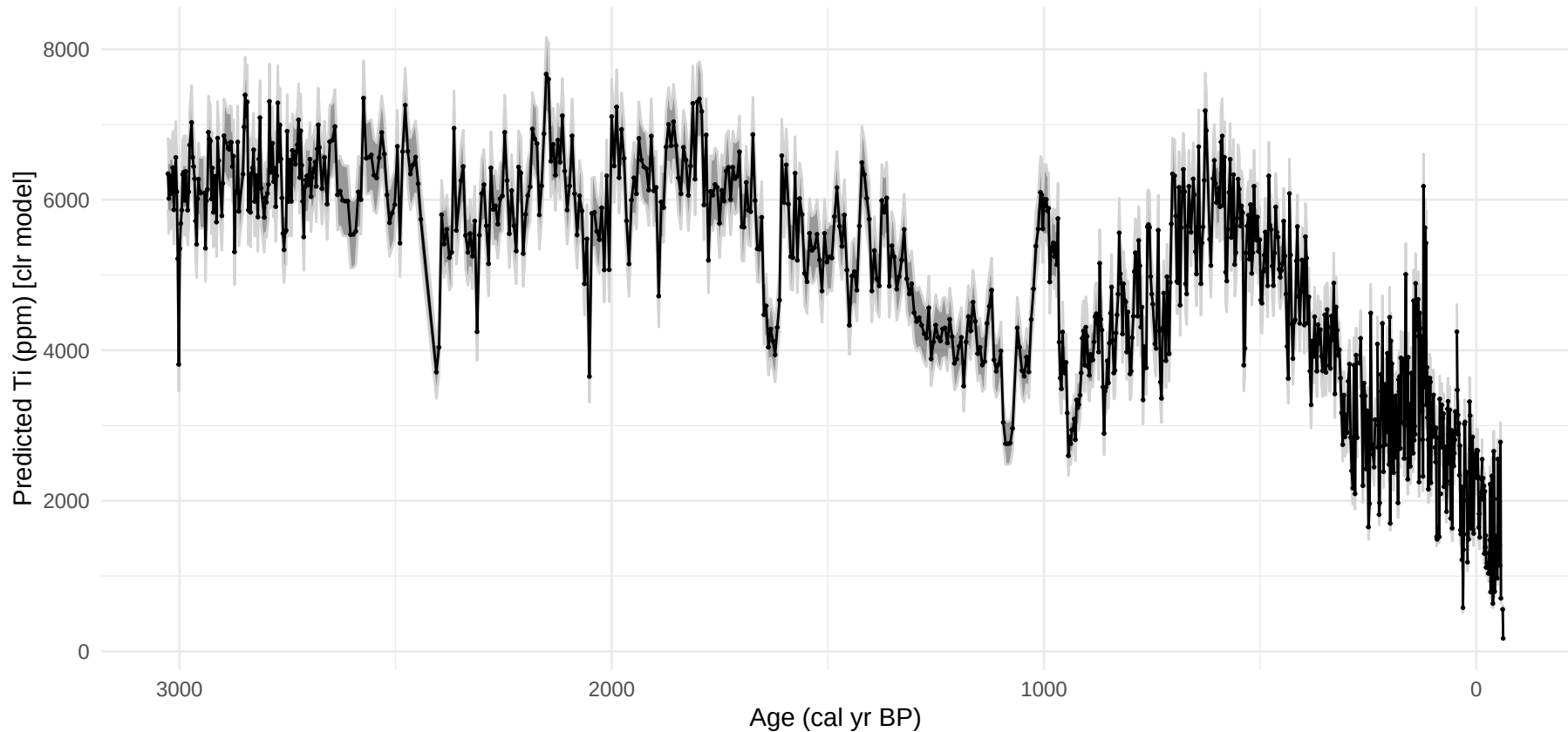
PB1: PLSR Ti Predictions with Confidence Interval (clr model)
