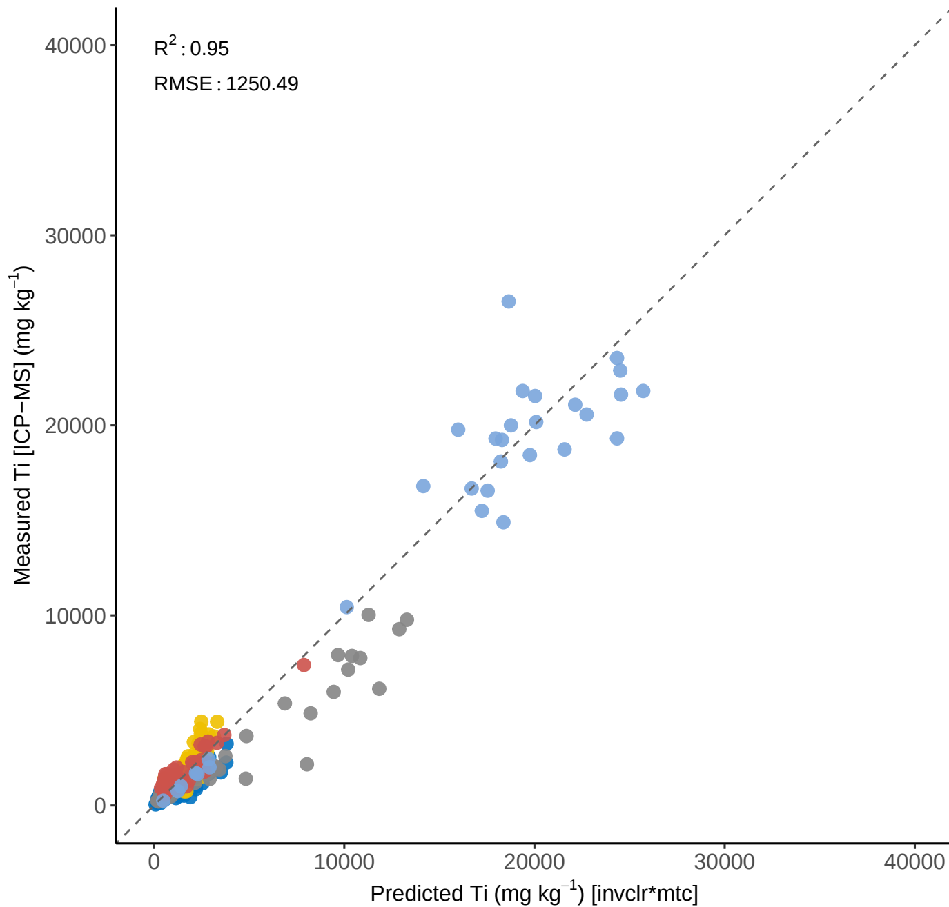
PLS Ti clr model: invclr*mtc to mg kg -1
