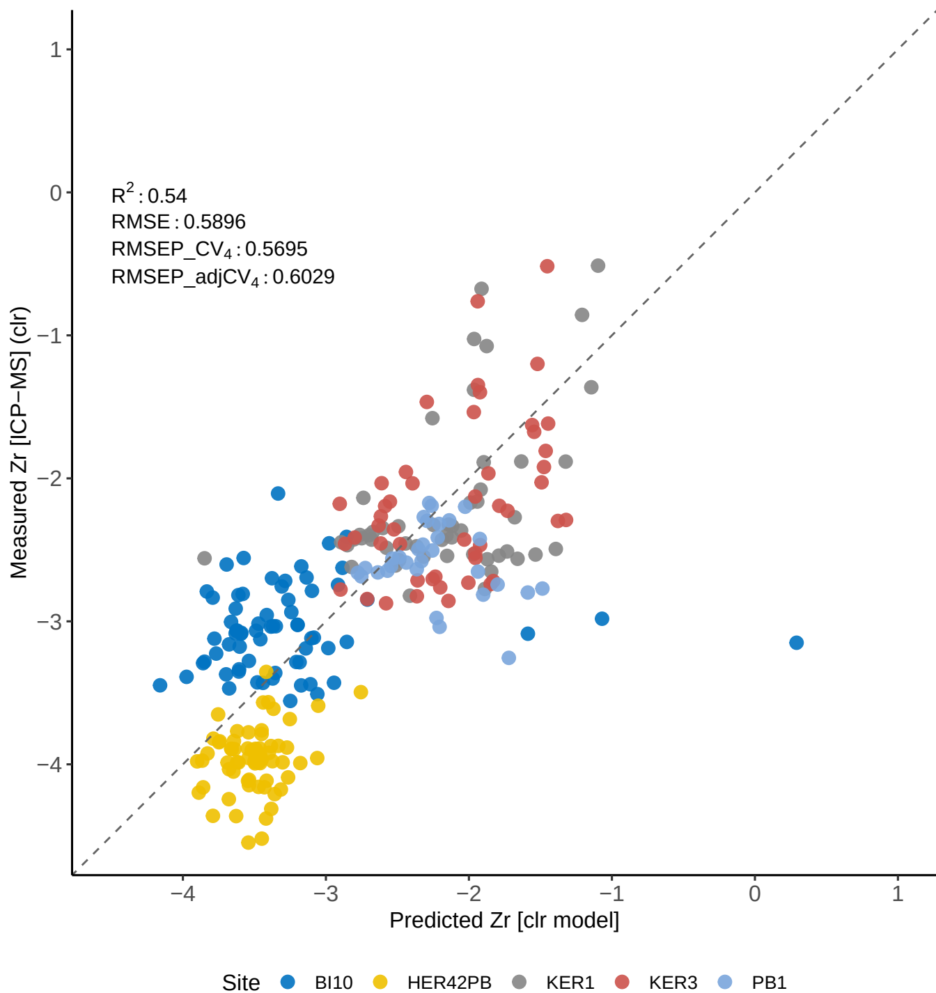
PLSR: Measured vs Predicted Zr: clr model
