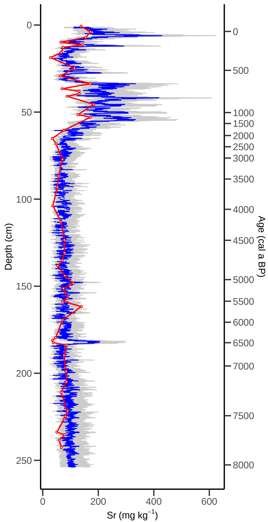
KER1: PLSR Sr Predictions with Confidence Interval
