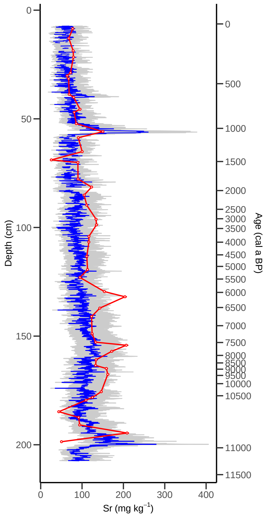
KER3: PLSR Sr Predictions with Confidence Intervals
