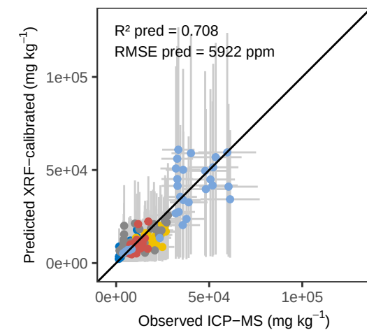
Ca PLS_LOO – External Validation
