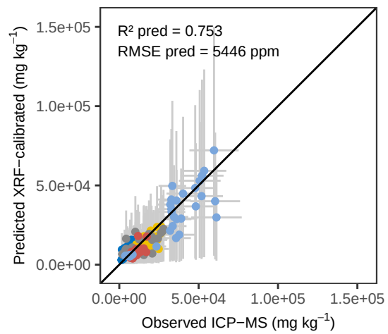
Ca WLS_weighted – External Validation
