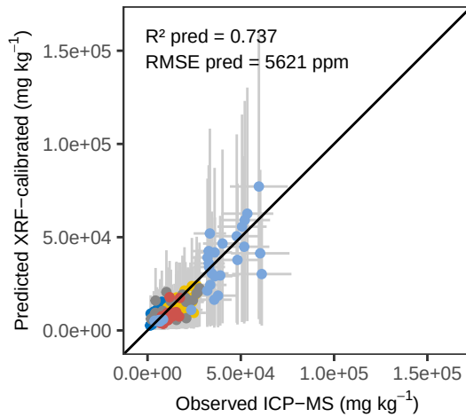
Ca Bayes – External Validation
